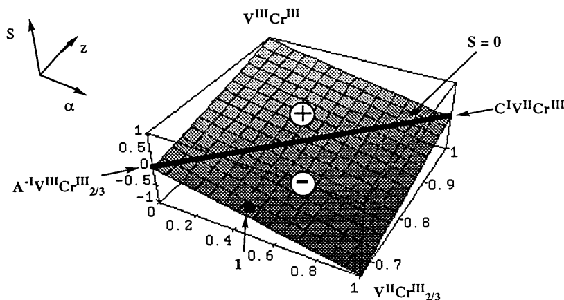
Fig. 8. Variation of the spin values S versus z and \alpha parameters for compounds C(I)_y V(II)_x V(III)_{1-x} [Cr(III)(CN)_6]_z \cdot nH_2O . 1 is in the part of the plane where the total spin has the same direction as the vanadium spins.
