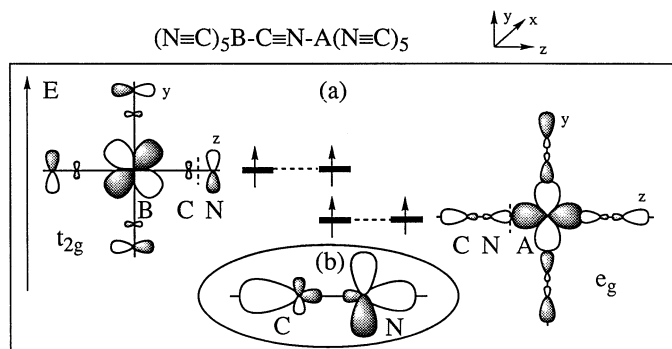
Fig. 5. Orthogonal magnetic orbitals in the (\text{NC})_5\text{B}-\text{C}\equiv\text{N}-\text{A}(\text{N}\equiv\text{C})_5 binuclear unit: (a) orthogonal t_{2g}(\text{B}) and e_g(\text{A}) orbitals left unchanged in the binuclear unit; (b) insert: spin density in two orthogonal p orbitals of nitrogen ( p_y and p_z ).
